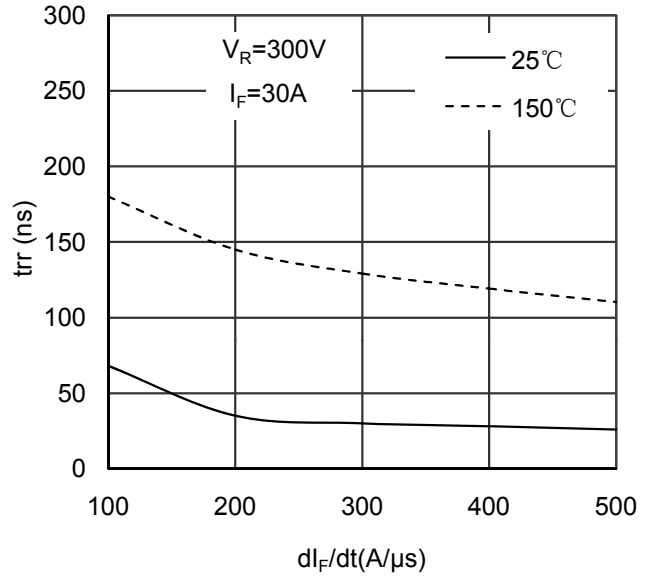
Figure 2. Reverse Recovery Time vs dl_F/dt
