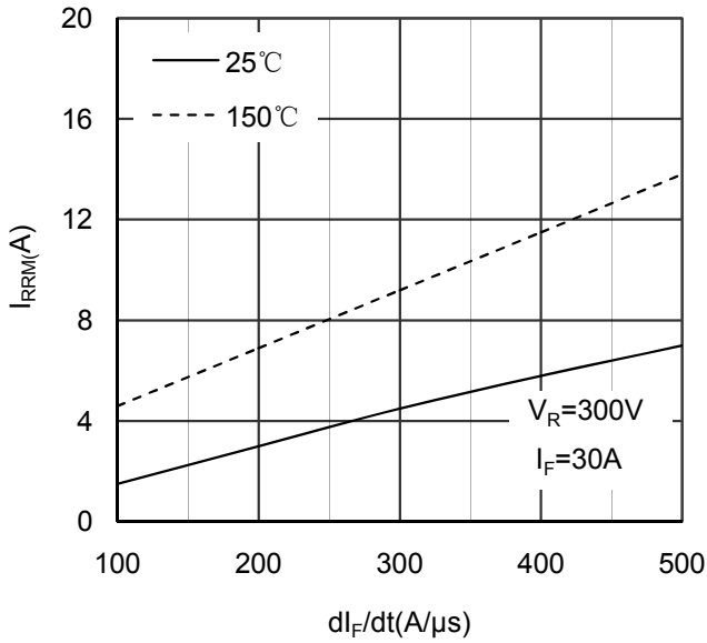
Figure 3. Reverse Recovery Current vs dl_F/dt
