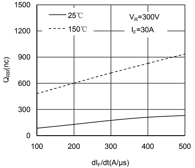
Figure 4. Reverse Recovery Charge vs dl_F/dt
