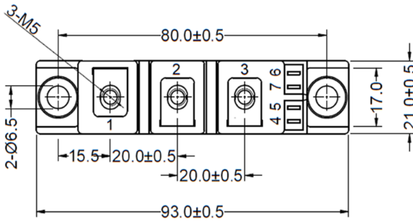
Dimensions in (mm) Figure 6. Package Outline
