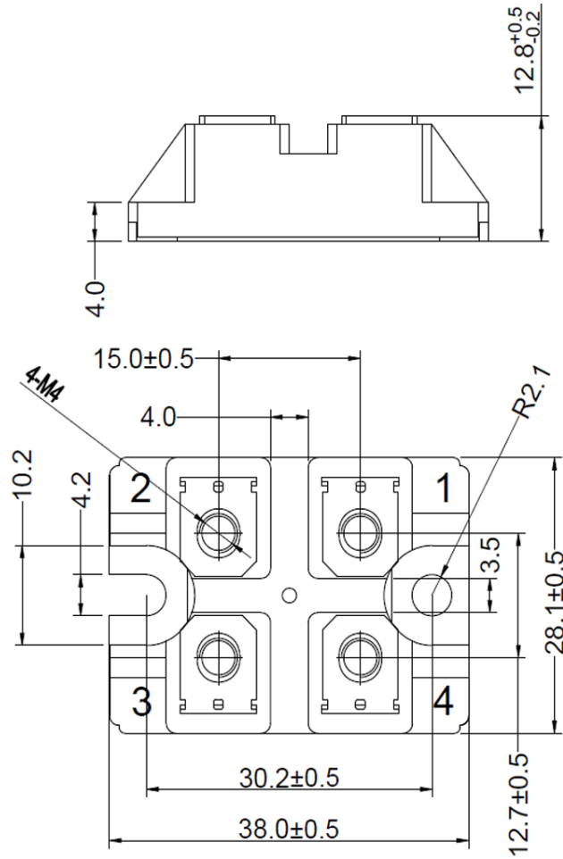
Dimensions in (mm) Figure 7. Package Outline
