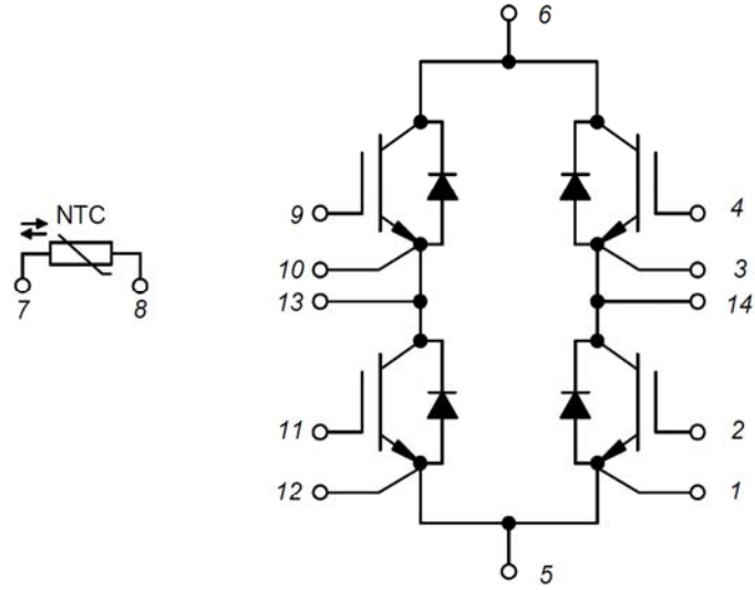
Figure 14. Circuit Diagram
