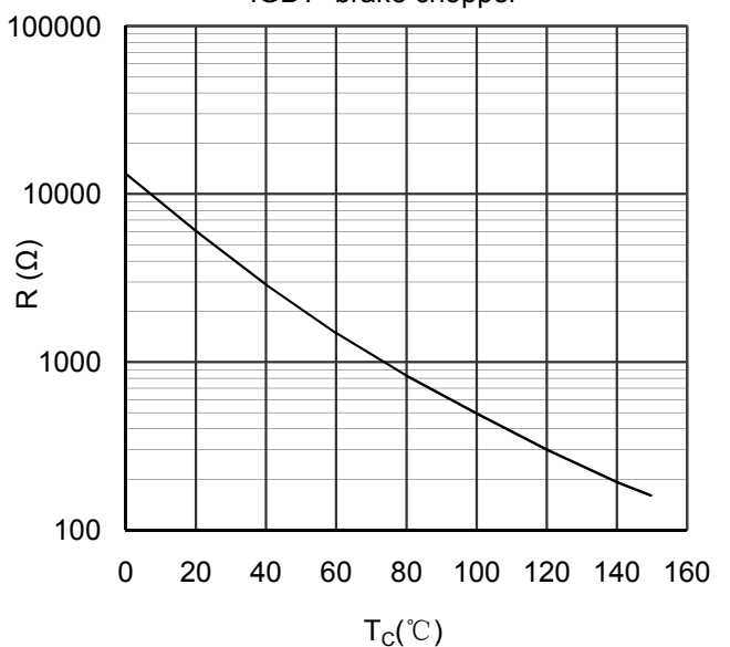
Figure 14. NTC Characteristics
