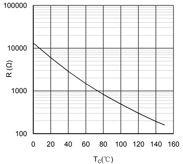
Figure 13. NTC Characteristics
