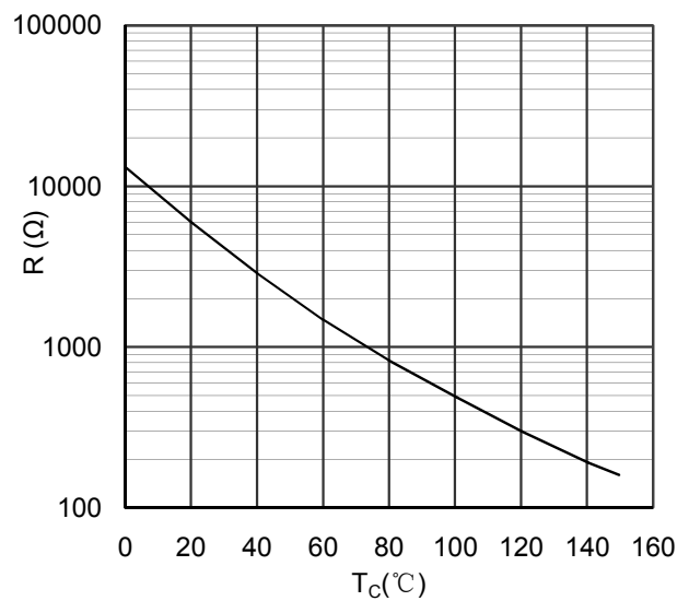
Figure 13. NTC Characteristics
