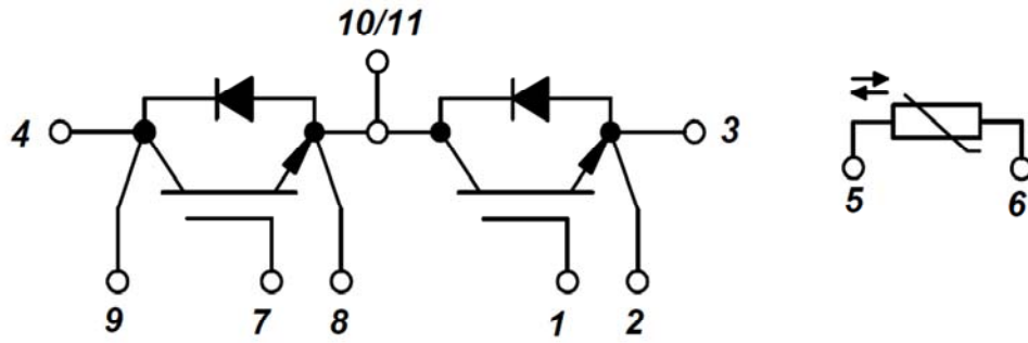
Figure 14. Circuit Diagram
