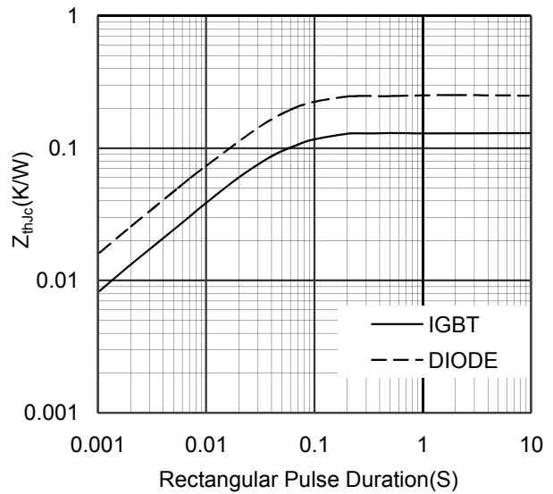
Figure 12. Transient Thermal Impedance of Diode-inverter and IGBT-inverter
