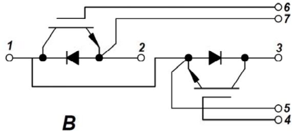
Figure 13. Circuit Diagram
