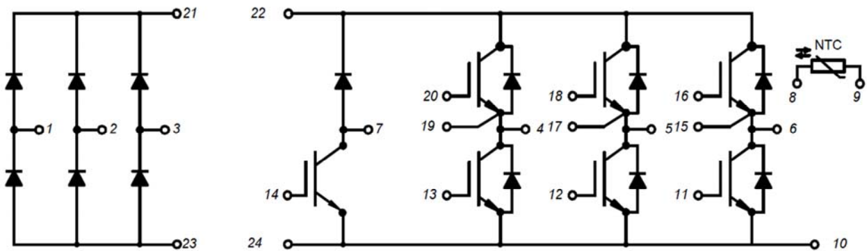
Figure 17. Circuit Diagram
