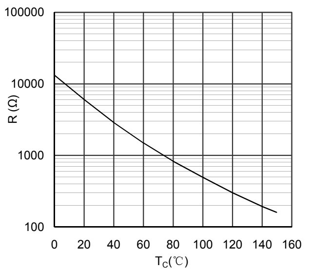
Figure 14. NTC Characteristics
