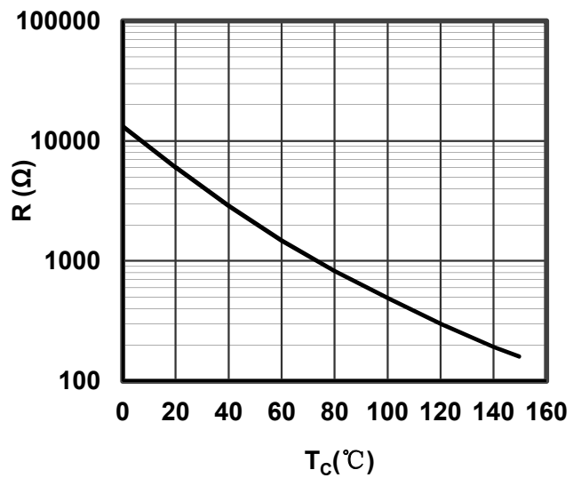
Figure 14. NTC Characteristics
