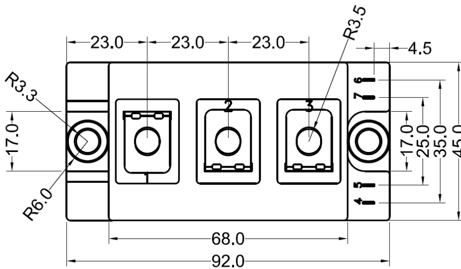
Dimensions (mm) Figure12. Package Outline
