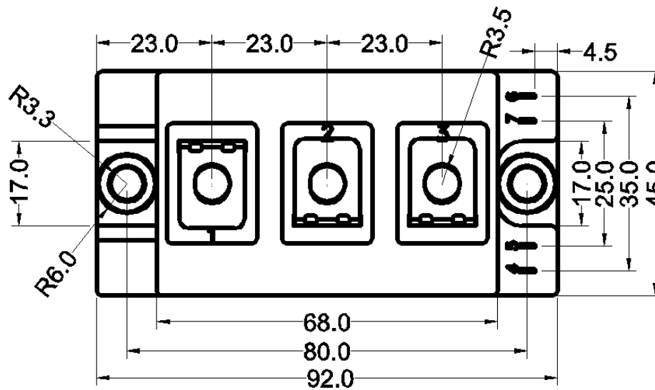
Dimensions (mm) Figure12. Package Outline
