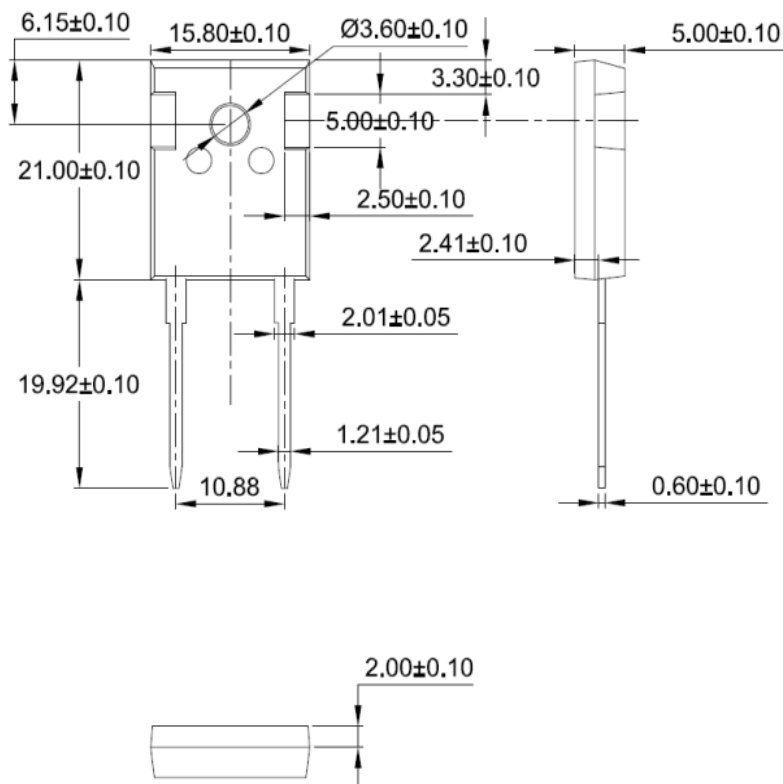
Figure 8. Package Outline
