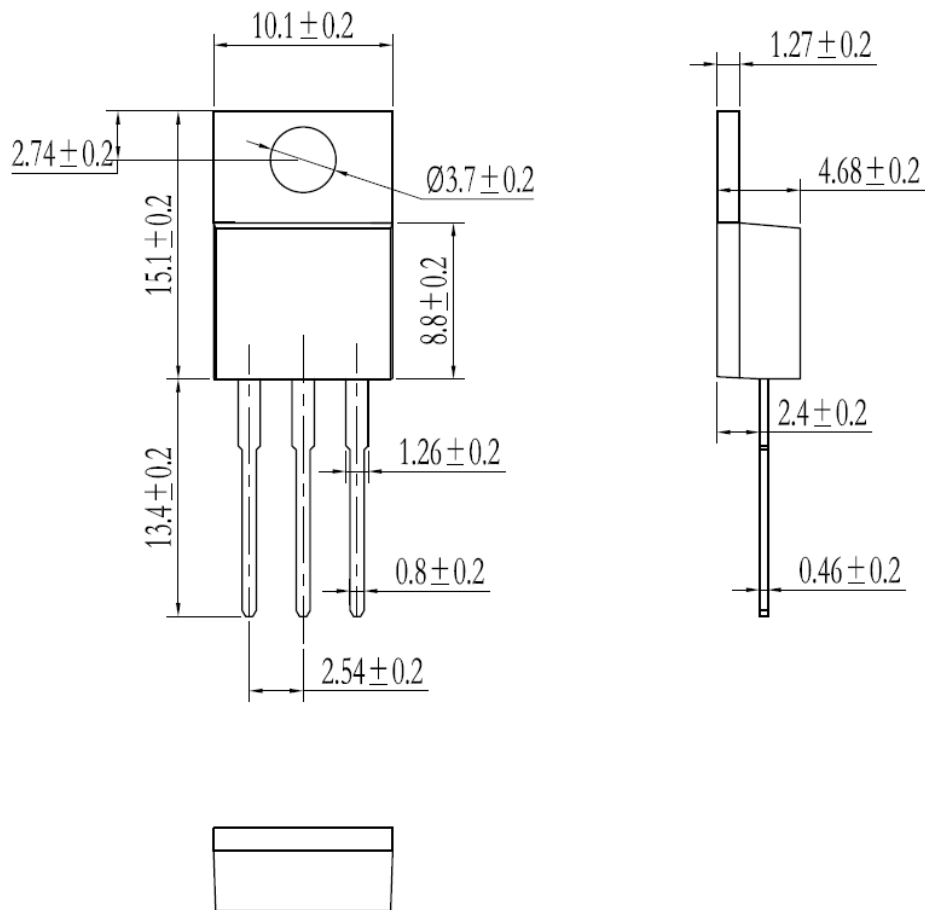
Dimensions in Millimeters Fig8. Package Outline
